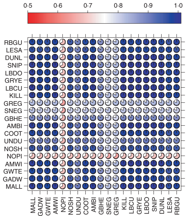
Fig. 8. A correlogram showing the frequency with which pairs of waterbird species both have zero abundance. The colour and the amount that a circle has been filled correspond to the proportion of observations with double zeros. The diagonal running from bottom left to top right represents the percentage of observations of a variable equal to zero. Four-letter acronyms represent different waterbird species. The top bar relates the colours in the graph to the proportion of zeros.
