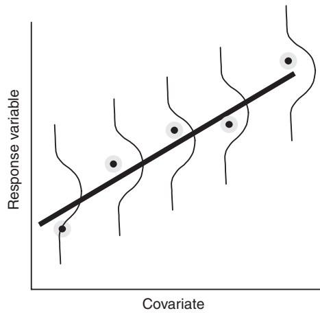
Fig. 6. Visualization of two underlying assumptions in linear regression: normality and homogeneity. The dots represent observed values and a regression line is added. At each covariate value, we assume that observations are normally distributed with the same spread (homogeneity). Normality and homogeneity at each covariate value cannot be verified unless many (> 25) replicates per covariate value are taken, which is seldom the case in ecological studies. In practice, a histogram of pooled residuals should be made, but this does not provide conclusive evidence for normality. The same limitations holds if residuals are plotted vs. fitted values to verify homogeneity.
